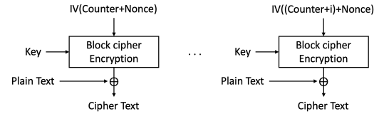
Fig. 2. Counter Operation mode of block cipher
